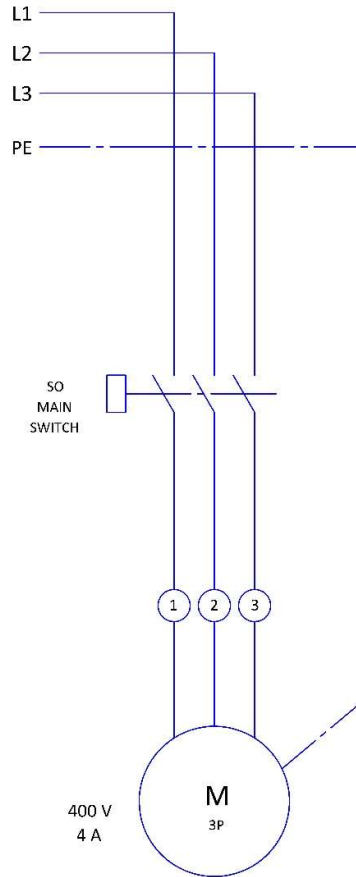
2.2 kW THREE-PHASE MOTOR
